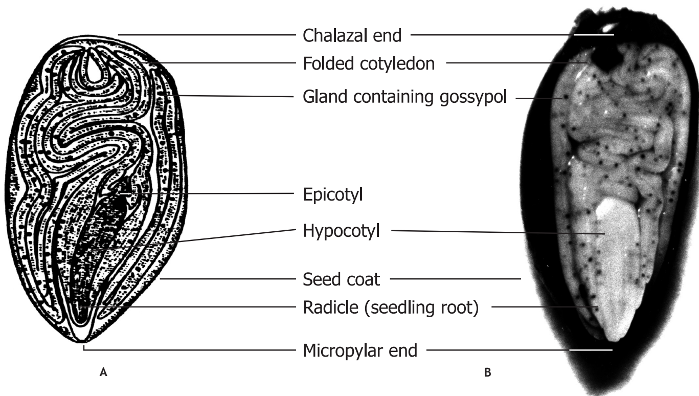
Figure 9. A diagram (A) and photo-micrograph (B) of a longitudinal section through a mature seed showing the seed coat and young embryo with folded cotyledons. (A, D. Oosterhuis; B, R.W. Seagull)
